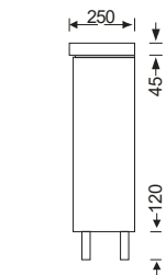
Manly SL50-25 (legs)
